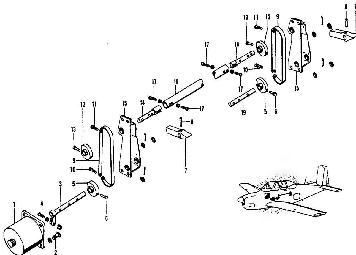
Figure 49. Ignition Switch Installation
