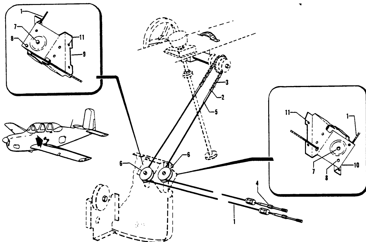
Figure 59. Aileron Trim Tab Control Cables
