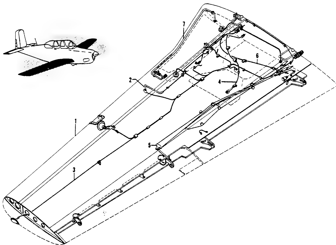
Figure 3. Wing Assembly
