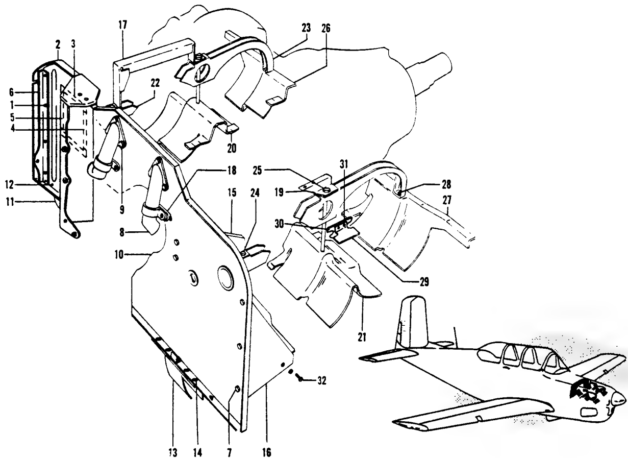
Figure 74. Engine Baffle Installation
