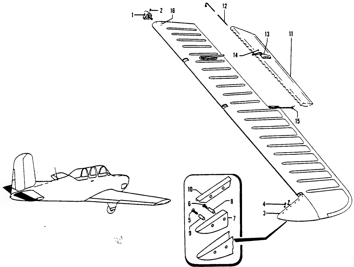
Figure 18. Elevator Assembly
