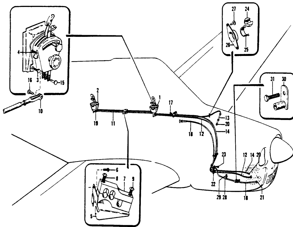
Figure 62. Engine Control Installation
