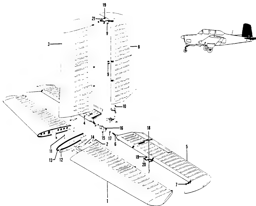
Figure 15. Empennage Installation
