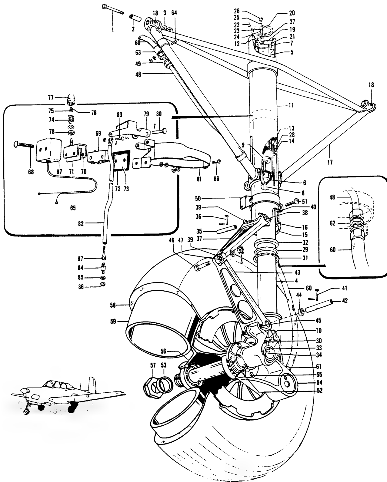
Figure 70. Main Alighting Gear Installation
